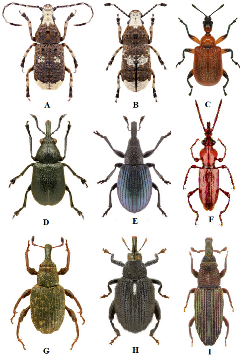
Figure 4. Some species of the weevils from State National Natural Park "Ulytau": Platytomos albinus , male (A) and female (B); Apoderus coryli (C); Auletobius sanguisorbae (D); Perapion affine (E); Eremoxenus chan (F); Orchestes jota (G); Dryophthorus corticalis (H); Bagous glabrirostris (I). Central Kazakhstan.
