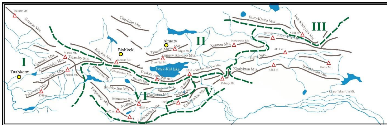
Fig. 1. Tian-Shan. I – West Tian-Shan, II – North Tian-Shan, III – Dzhungaria, IV – East Tian-Shan, V – Inner Tian-Shan, VI – Central Tian-Shan.
