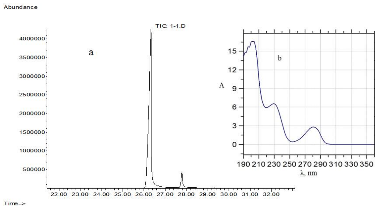
Fig. 1. HPLC chromatogram (a), UV spectrum and (b) of arctigenin extracted from Arctium lappa fructus
