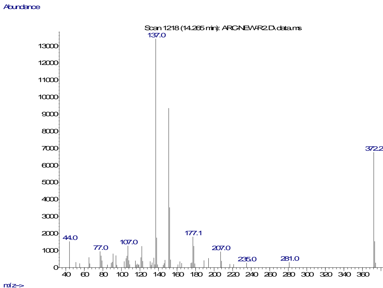
Fig. 2. Mass spectrum of arctigenin extracted from Arctium lappa fructus
