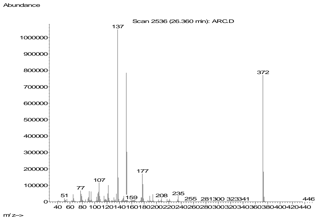
Fig. 4. Mass spectrum of standard substance arctigenin
