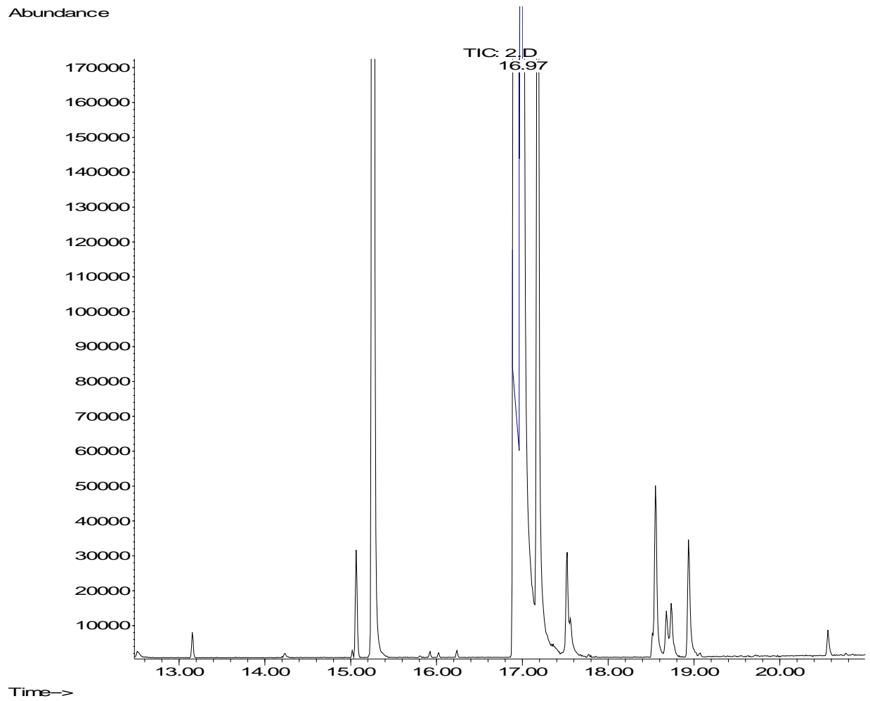
Fig. 6. HPLC chromatogram of Arctium tomentosum ethanol extract
