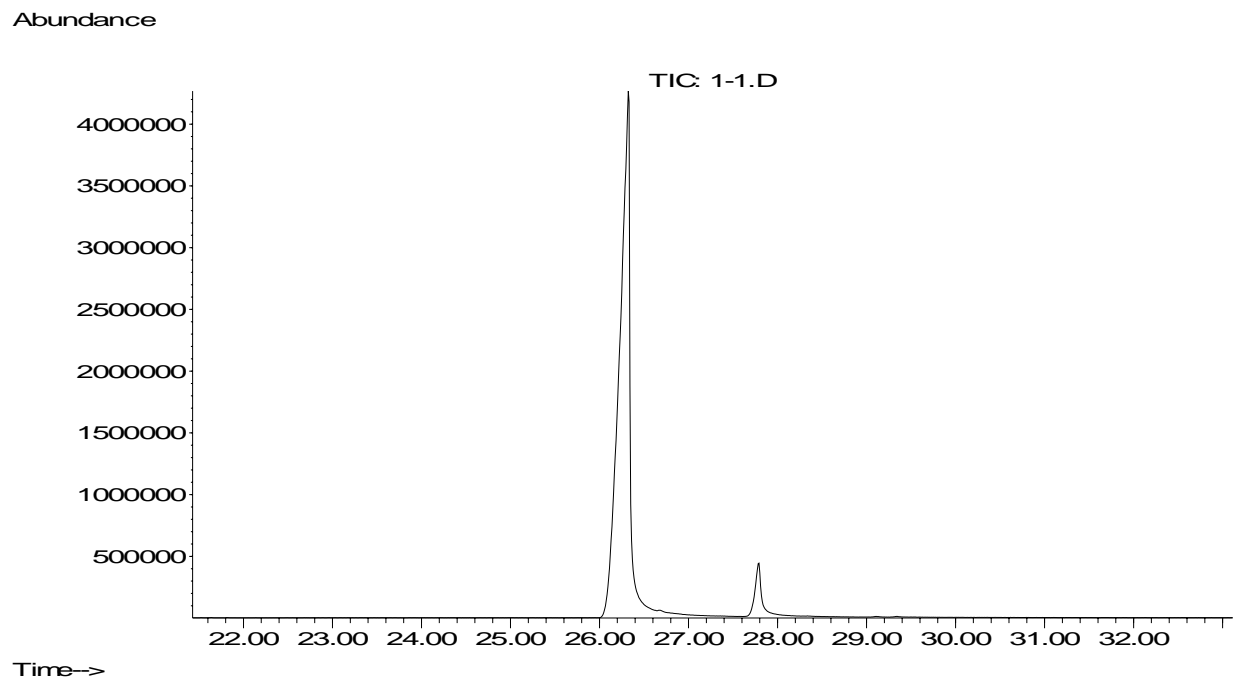
Fig. 3. HPLC chromatogram of standard substance arctigenin
