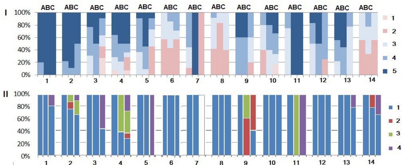
Figure 7. Anatomical structure of the stem and leaf (lower leaf sheaths) epidermis of Poa botryoides . A - stem under panicle; B - stem under the node (in the lower part); C - sheaths of lower leaves. Locations of the studied populations: 1 - Buryatia; 2 - Chita region; 3 - Khakasia; 4 - Buryatia; 5 - Baikal; 6 - Irkutsk region; 7 - Buryatia; 8 - Magadan region; 9 - south of the Krasnoyarsk district; 10, 11 - Chita region; 12 - Khakasia; 13 - south of the Krasnoyarsk district; 14 - Khakasia. I Morphological types of trichomes: a - surface with rare crown cells (rarely completely smooth); b - numerous crown cells; c - rare prickles or bristles appear; d - prickles or bristles of medium density, often arranged in rows; e - prickles or bristles dense. Crown cells are pink, prickles are blue. II Direction of trichomes; a - upwards; b - downwards; c - directed up and down; d - directed perpendicular to the surface of the stem.
