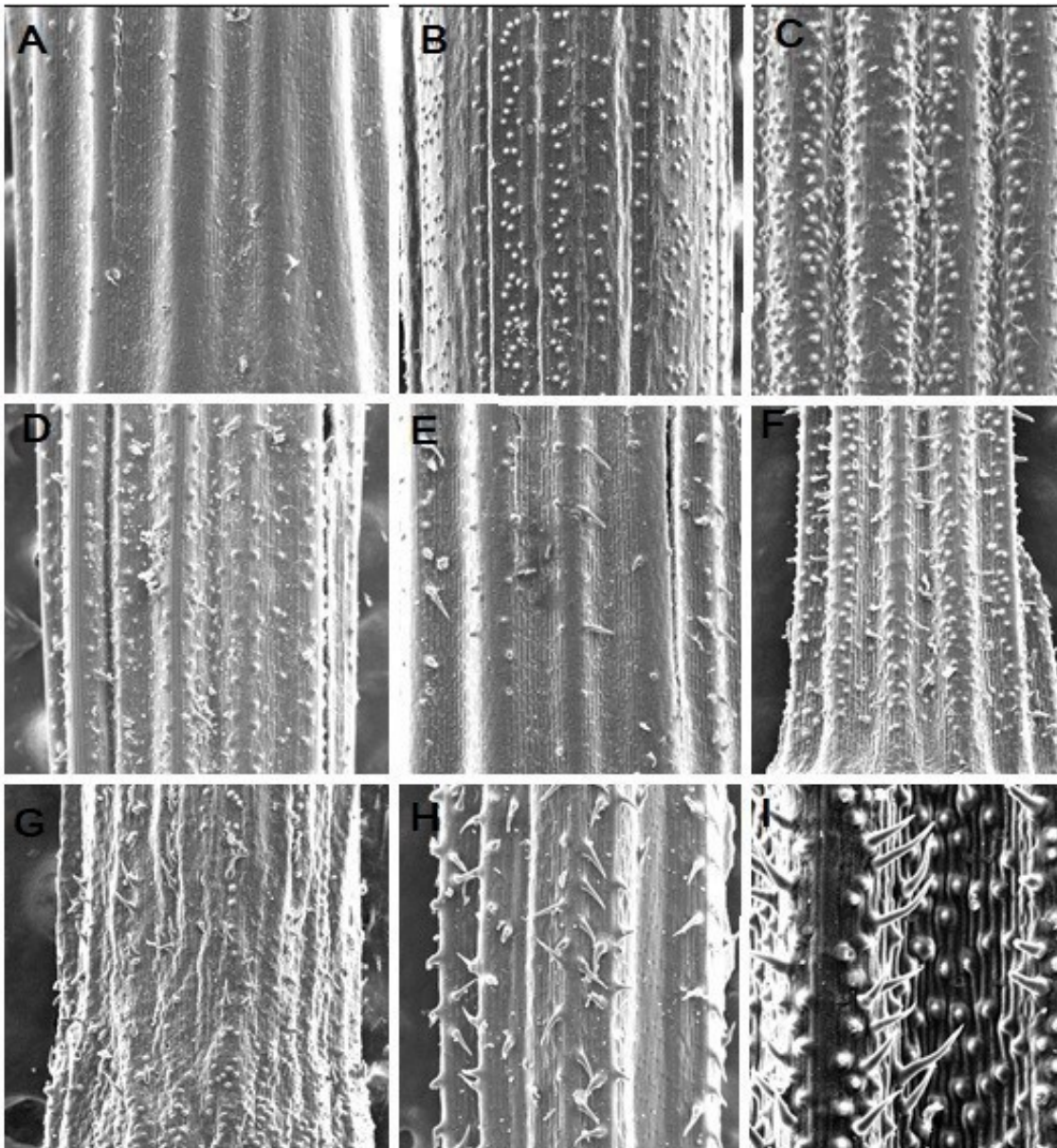
Figure 4. Sculptural elements of the leaf sheaths epidermis above the nodes. A-H ( \times 100 ). I ( \times 300 ). Character states: A - individual crown cells (rarely almost completely smooth); B, C - numerous crown cells; D, E - in addition to crown cells, random and rare pricles appear; F, G - pricles of medium density, usually arranged in rows; H, I - dense pricles.
