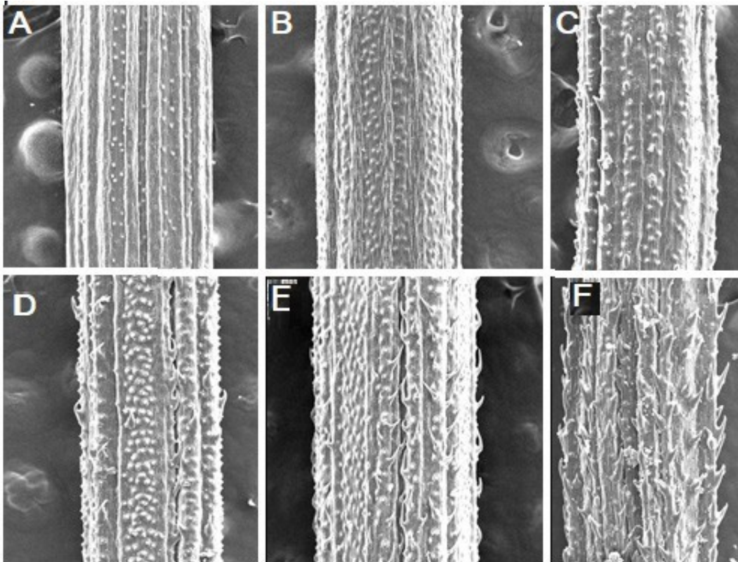
Figure 2. Sculptural elements of the stem epidermis under the panicle ( \times 110 ). Character states: A - individual crown cells (rarely almost completely smooth); B - numerous crown cells; C - in addition to crown cells, random and rare pricles appear; D - pricles of medium density, usually arranged in rows; E, F - dense pricles.
