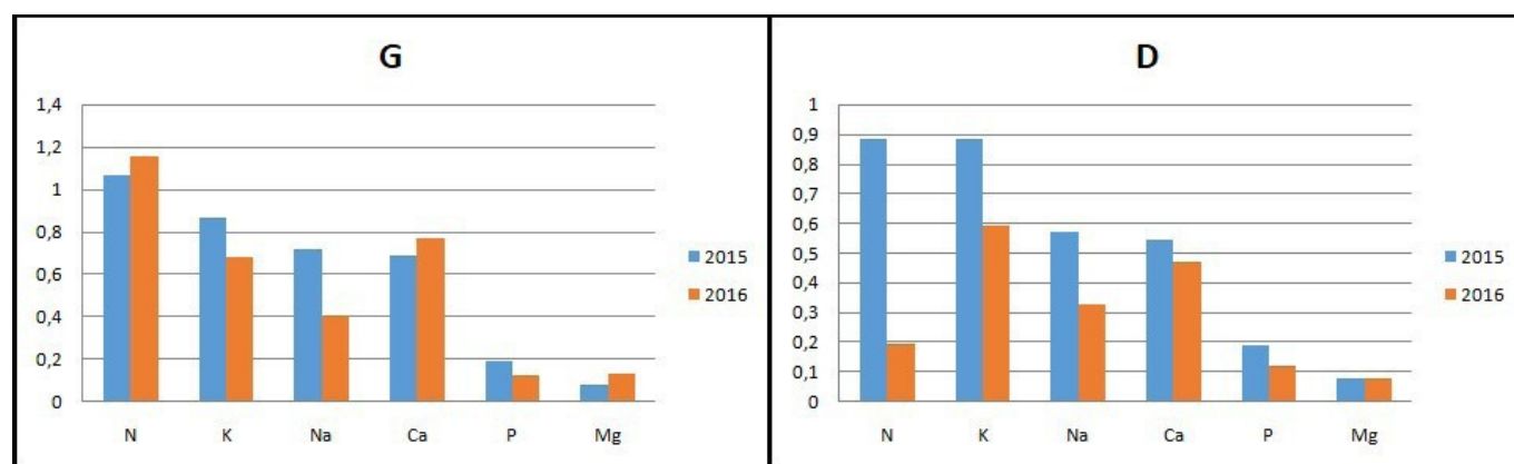
Figure 2. The average content of mineral elements in the above-ground phytomass of the forb-fescue-feather grass steppe ( Stipa zaleskii , S. lessingiana , Herbae stepposae ) with Helictotrichon desertorum and petrophytous elements of the community. G – living above-ground phytomass, D – above-ground dead phytomass.
