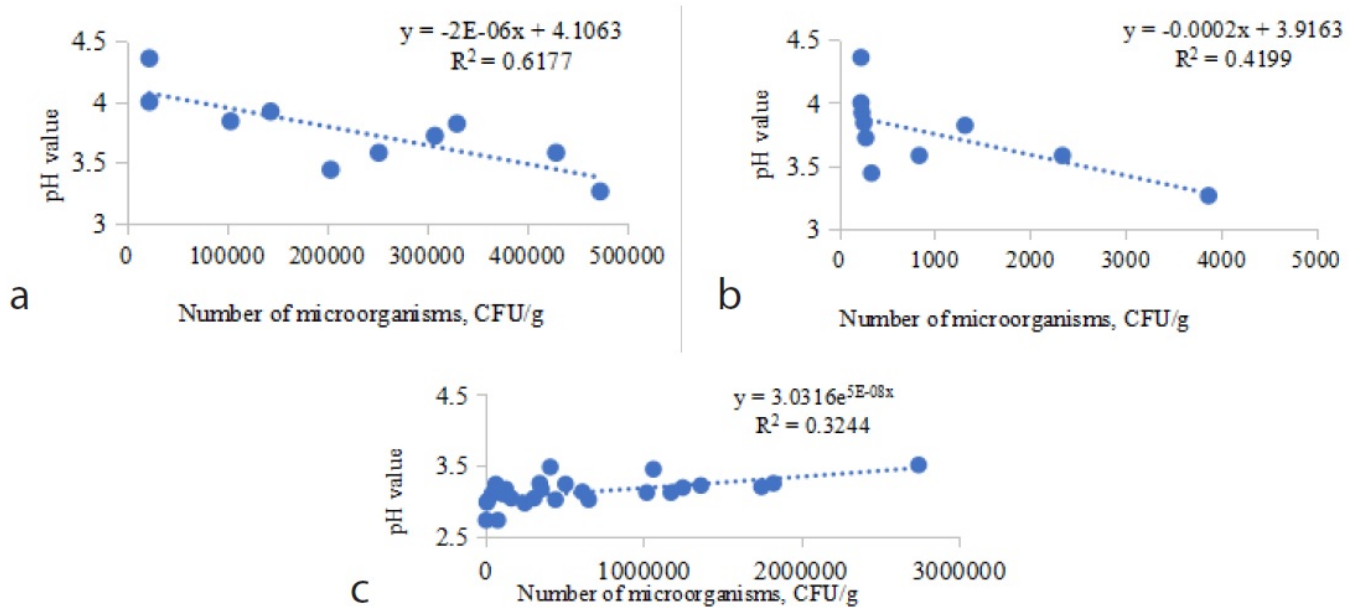
Figure 4. The relationship between the number of ammonifying microorganisms (a), saccharolytic micromycetes (b) in the permafrost layer, and oligotrophic microorganisms (c) in the active layer of peat with the pH value.
