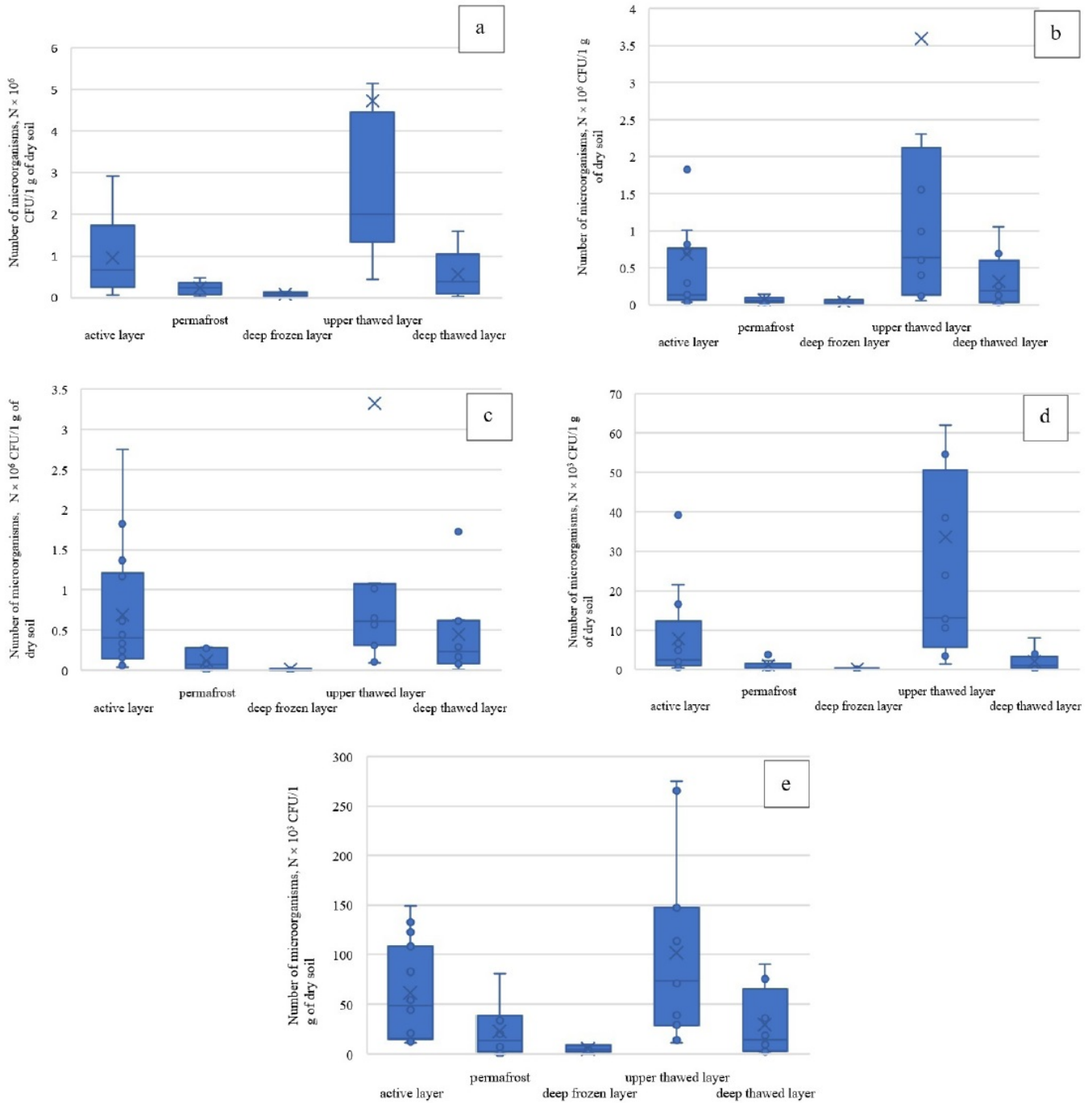
Figure 3. Number of microorganisms of various ecological and trophic groups in the active, frozen and thawed soil layers: ammonifying (a), amylolytic (b), oligotrophic (c), saccharolytic micromycetes (d), humus-destroying (e).
