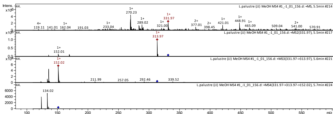
Fig. 4. CID spectrum of 11-Hydroxy- \Delta^9 -Tetrahydrocannabinol (11-OH-THC) from L. palustre , m/z 331.97
