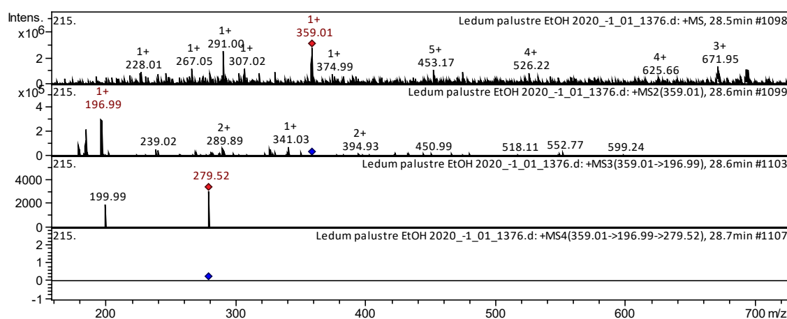
Fig. 5. CID spectrum of Cannabidiolic acid from L. palustre , m/z 359.01
