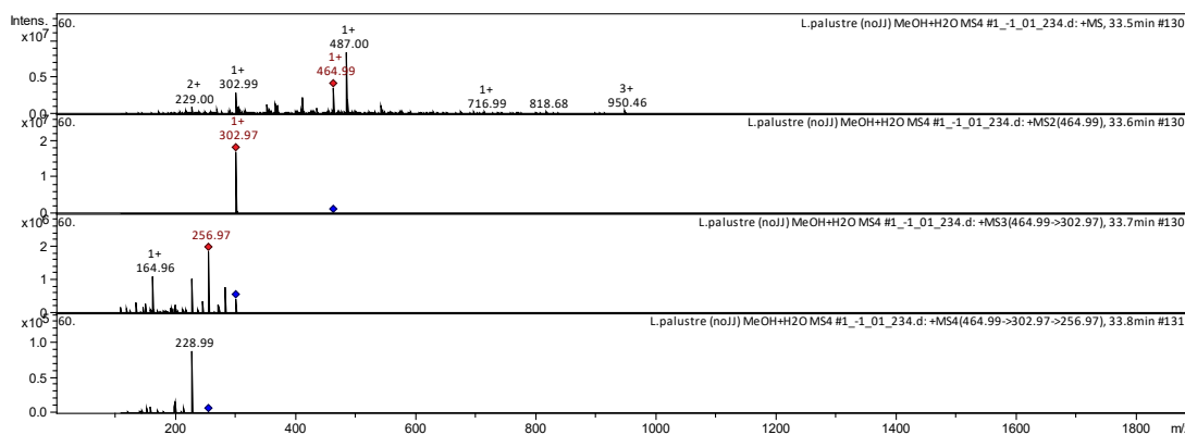
Fig. 6. CID spectrum of Hyperoside from L. palustre , m/z 464.99
