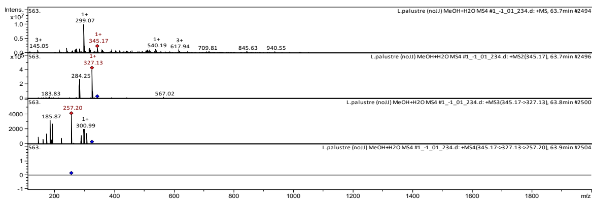
Fig. 2. CID spectrum of 11-nor-9-carboxy-THC from L. palustre , m/z 345.17
