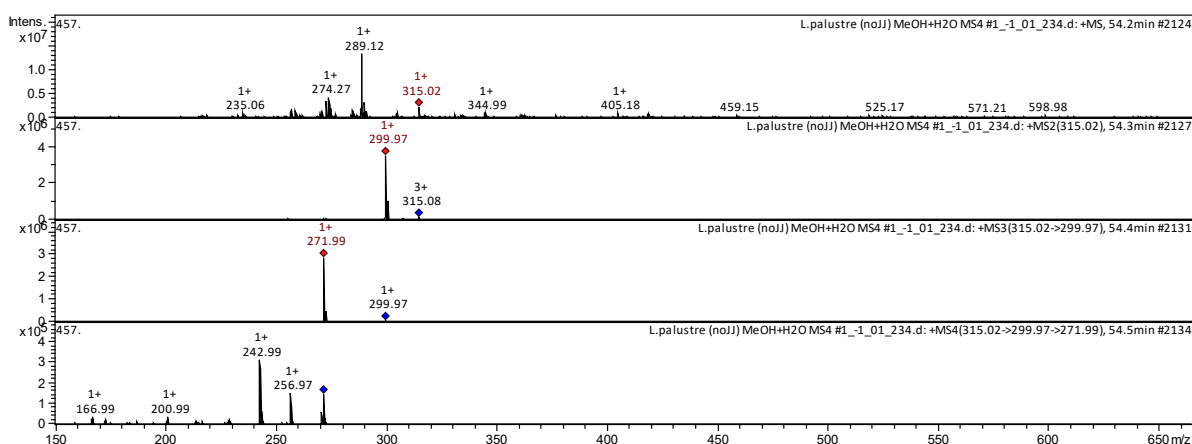
Fig. 3. CID spectrum of \Delta^9 -Tetrahydrocannabinol from L. palustre , m/z 315.02
