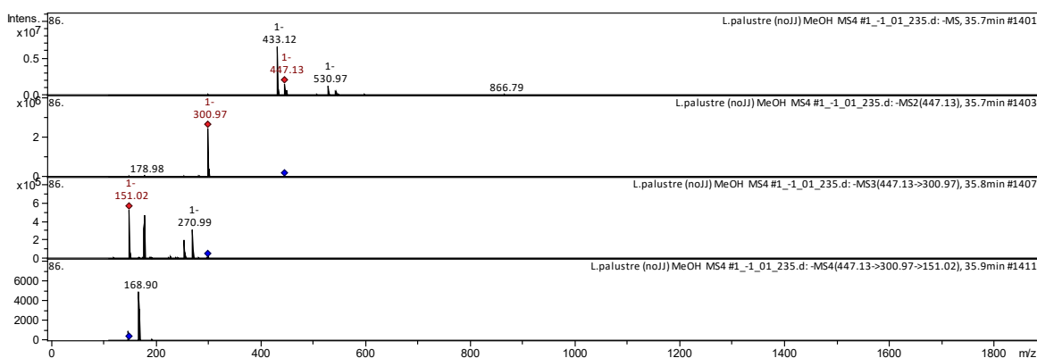
Fig. 7. CID spectrum of Quercitrin from L. palustre , m/z 447.13
