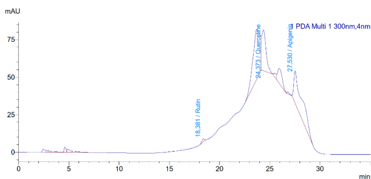
Fig. 1. Chromatogram for the determination of polyphenols in the sample extract
