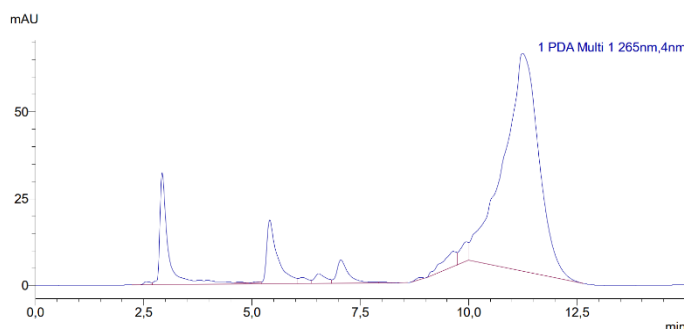
Fig. 3. Chromatogram for the determination of Vitamin C in the sample (aqueous extract of Cinnamomum verum )
