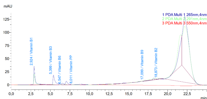
Fig. 2. Chromatogram for the determination of vitamins in the sample (aqueous extract of Cinnamomum verum )
