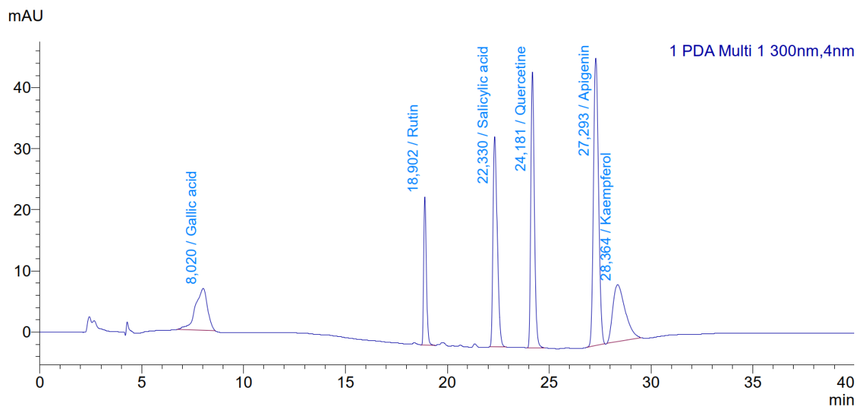
Fig. 1. Chromatogram of standards at 300 nm
