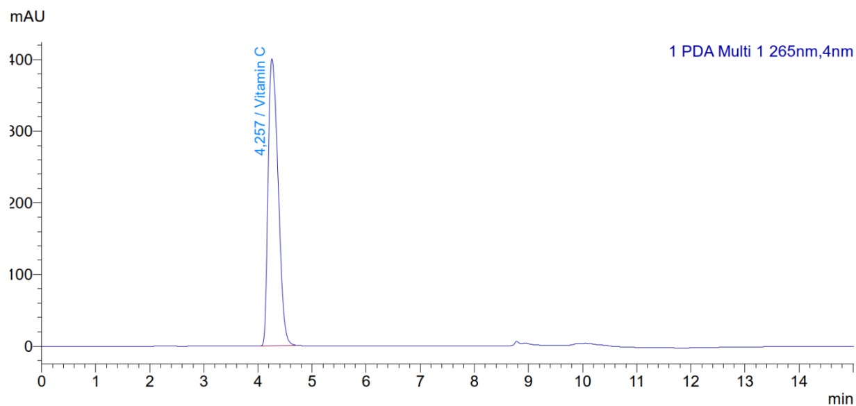
Fig. 2. Chromatogram of the Vitamin C standard solution
